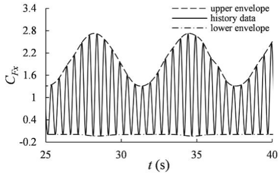
(b) With surging motion ( U=1 m/s, \lambda = 2.5 , \omega_x = 1 rad/s , A_x = 0.2 m )
