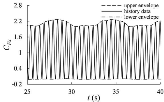
(c) With swaying motion ( U=1 m/s, \lambda = 2.5 , \omega_y = 1 rad/s , A_y = 0.2 m )
